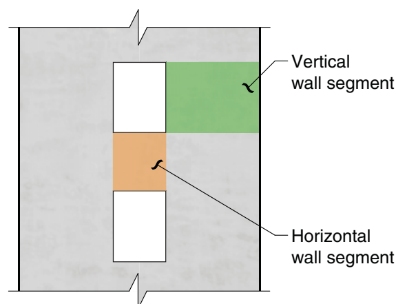
Fig. R18.10.4.5—Wall with openings.
