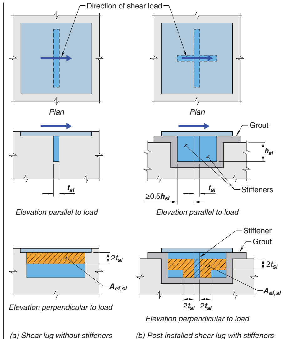
Fig. R17.11.2.1.1 —Examples of effective bearing areas for attachments with shear lugs.
