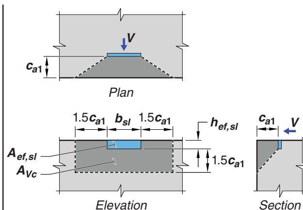
Fig. R17.11.3.1—Example of A_{vc} for a shear lug near an edge.
