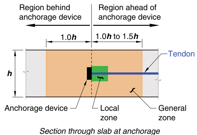
Fig. R25.9.1.1a—Local and general zones.
