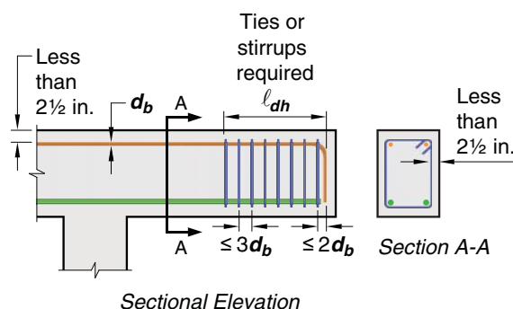
Fig. R25.4.3.4—Concrete cover according to 25.4.3.4.
