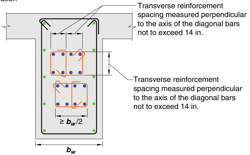
Fig. R18.10.7a —Confinement of individual diagonals in coupling beams with diagonally oriented reinforcement. Wall boundary reinforcement shown on one side only for clarity.
