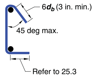
(a) single-leg stirrup or bar
