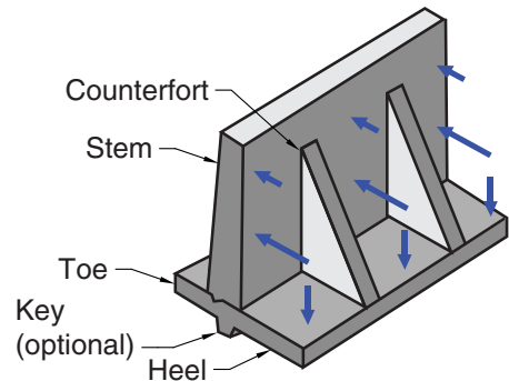
Counterfort/buttressed
