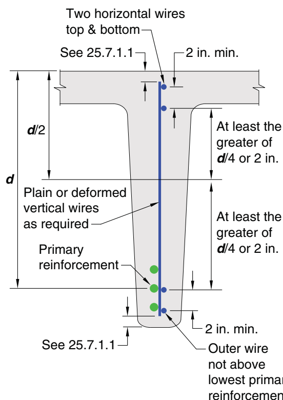
Fig. R25.7.1.5 —Anchorage of single-leg welded wire reinforcement for shear.
