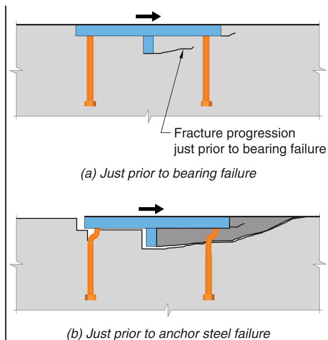
Fig. R17.11.1.1b —Bearing failure and subsequent anchor steel failure for embedded plate with shear lug (if concrete breakout is not applicable)
