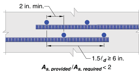
Fig. R25.5.4.1 —Lap splices of plain welded wire reinforcement where A_{s, provided}/A_{s, required} < 2 .
